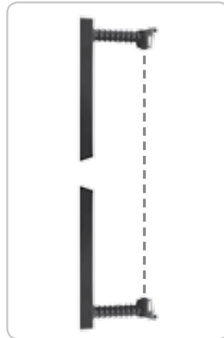
WIRELESS PHOTOCELLS SUBSTITUTING THE SAFETY STRIP VERTIGO Wi-Fi 8 code ACG8042 VERTIGO Wi-Fi 10 code ACG8043
